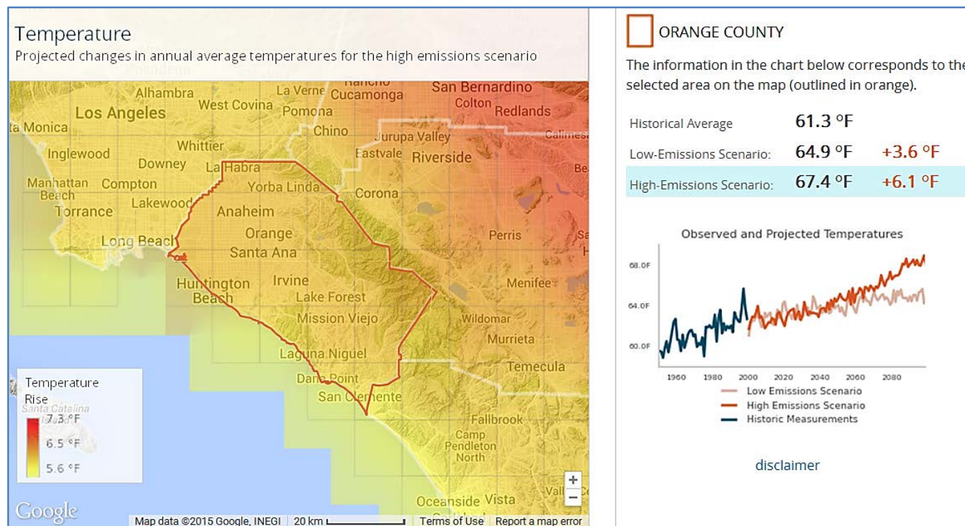
Figure 2. Projected changes in annual average temperature in future carbon emissions scenarios, Orange County, 2099 6
