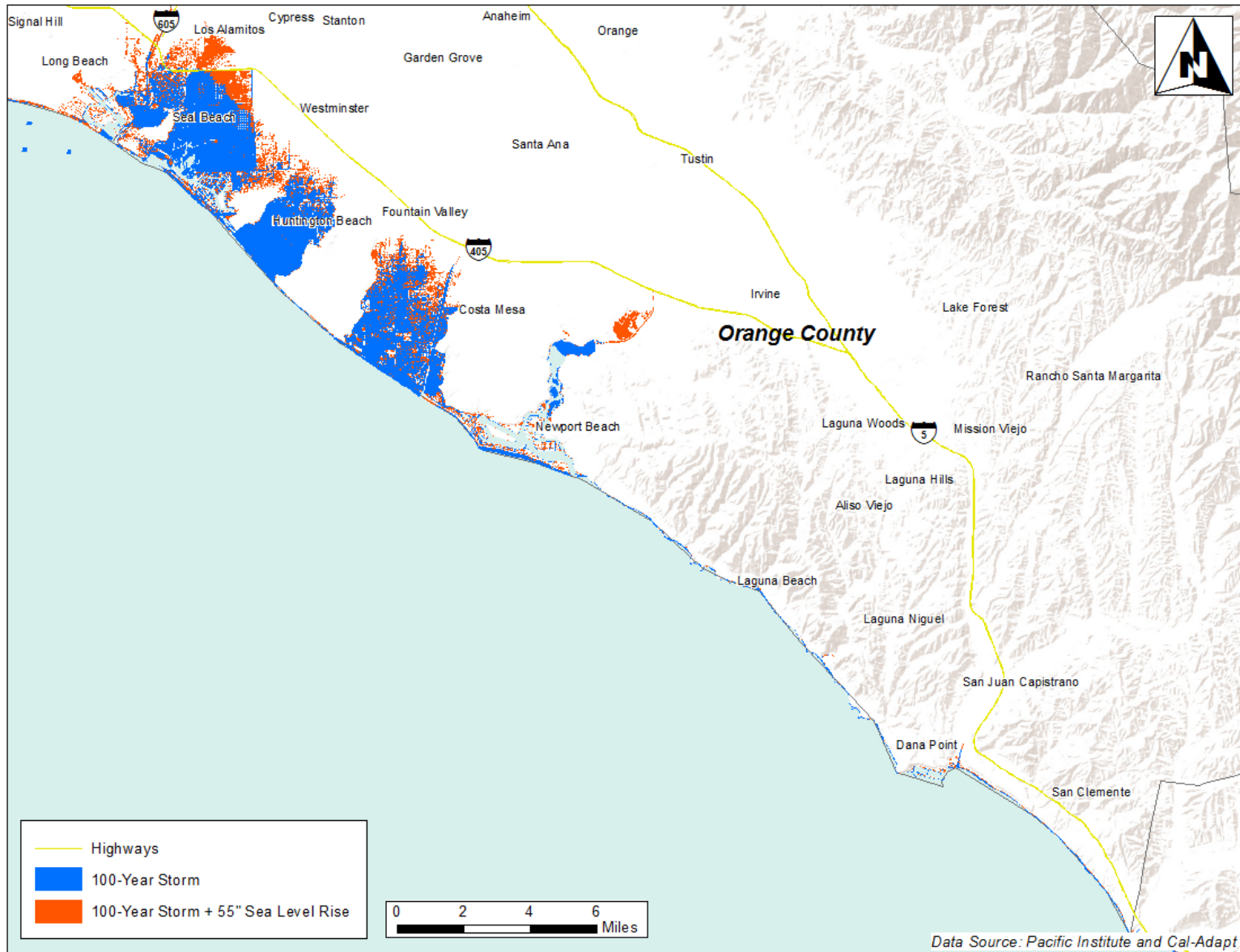
Figure 5. Baseline inundation areas for a 100-year flood (2000) and modeled scenario with additional 55 inches of sea level rise (2100), Orange County 6 Note: Current projections are 66 inches above sea level. 7
