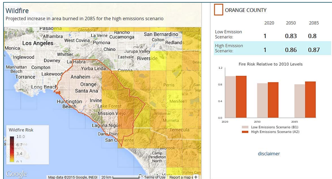
Figure 4. Relative increase in wildfire acreage in future carbon emission scenarios, Orange County 6
