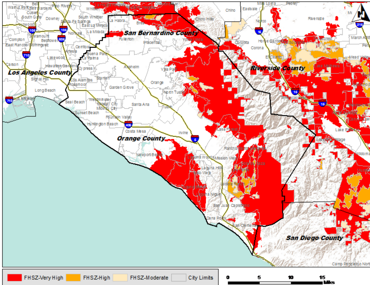
Figure 3. Current Fire Hazard Severity Zones (FHSZ), Orange County, 2007 9
